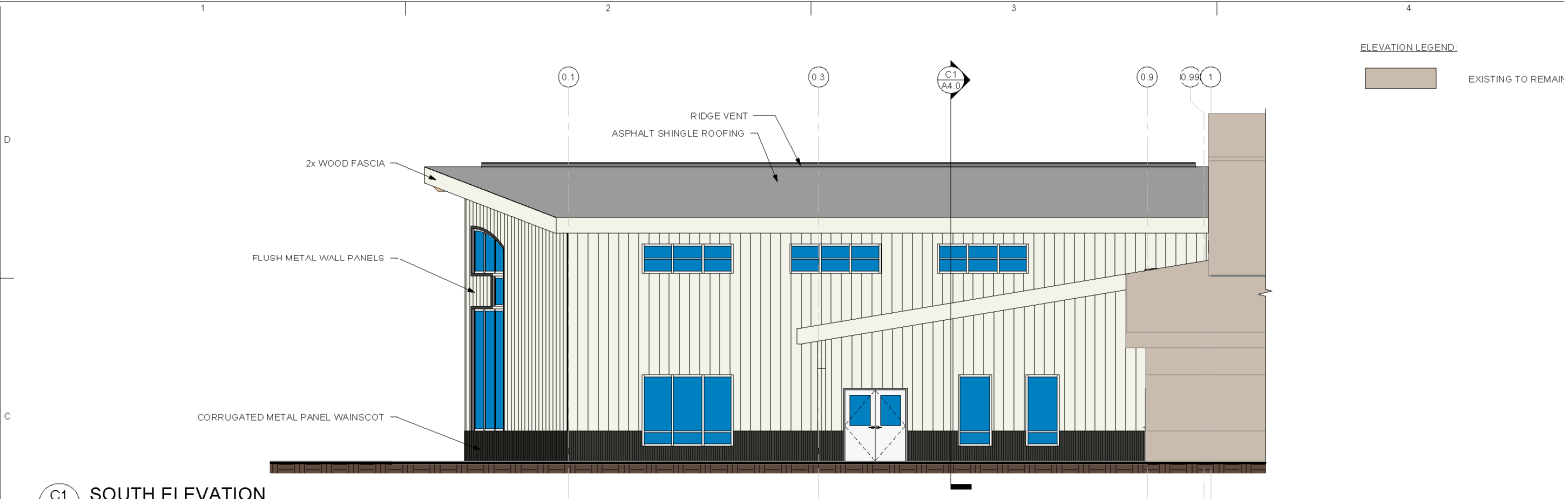
C1 A3.1 SOUTH ELEVATION 3/16" = 1'-0" (22x34), 3/32" = 1'-0" (11x17)
